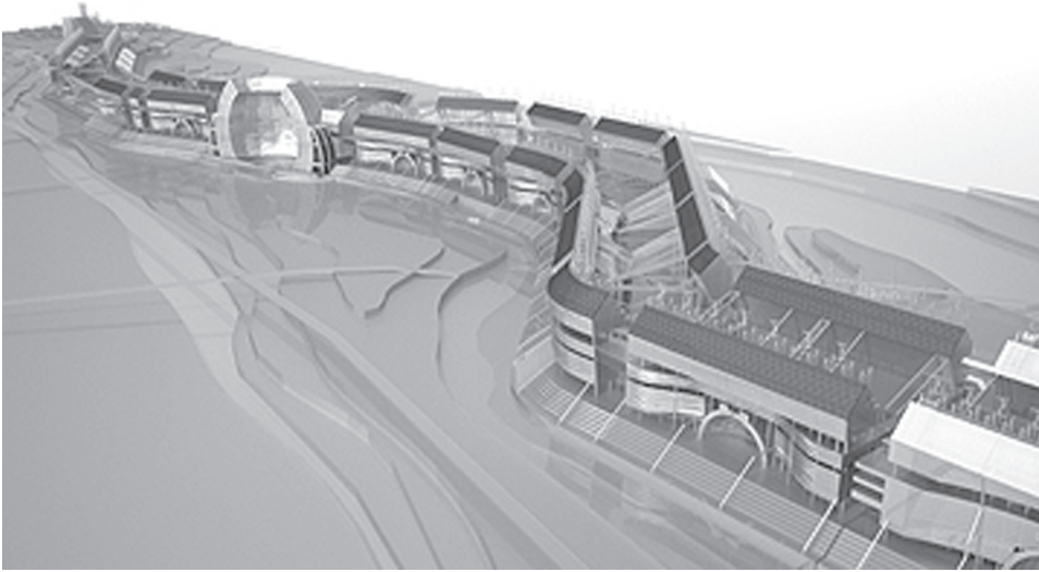
Figure 742-5. LEAN LINEAR CITY will be connected to even larger nodes, like the NUDGING SPACE Arcology. (3D rendering: Youngsoo Kim)
