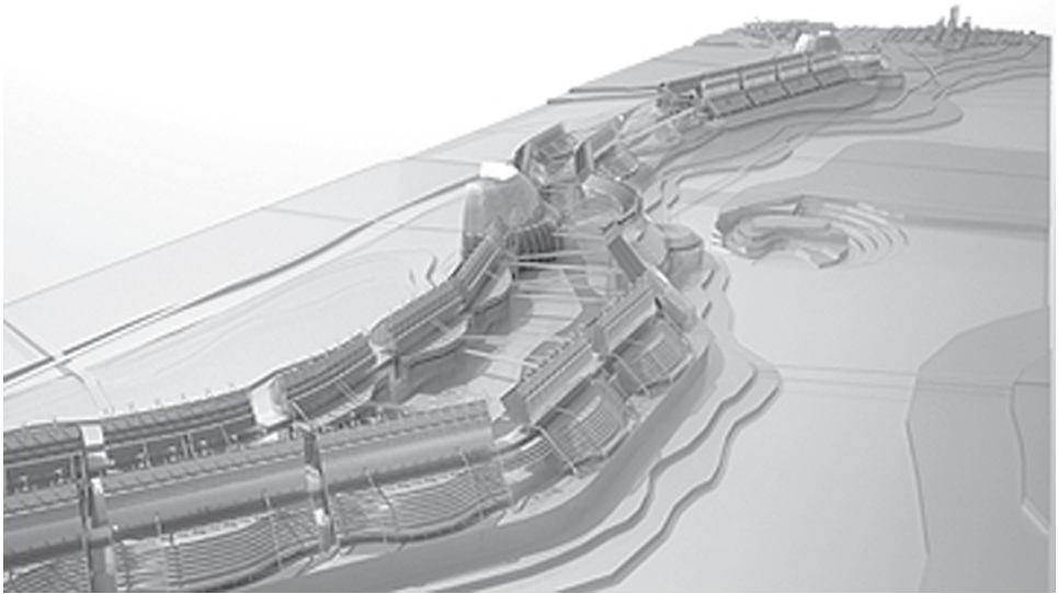
Figure 742-6. Two main parallel structures are built of modules measuring 150 meters (500 feet) in length. A climate-controlled volume constitutes the inner park defined by the two structures. (3D rendering: Youngsoo Kim)
