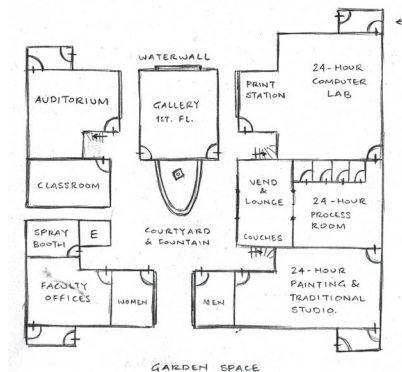
Figure 5581-1. Plan of first floor.
